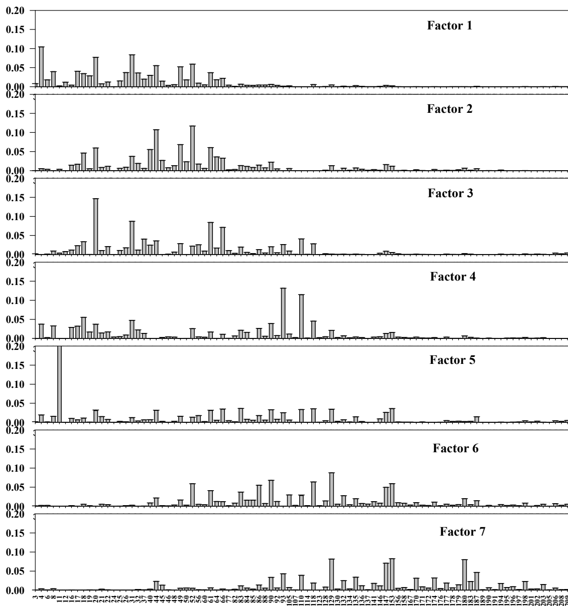
Figure 5.3. Normalized congener patterns of the seven resolved source profiles (factors). PCB congener numbers on the x-axis are plotted vs. their fractional contribution to the sum of PCBs on the y-axis. Error bars stand for the calculated standard deviation of the fractional contribution of each PCB congener.
