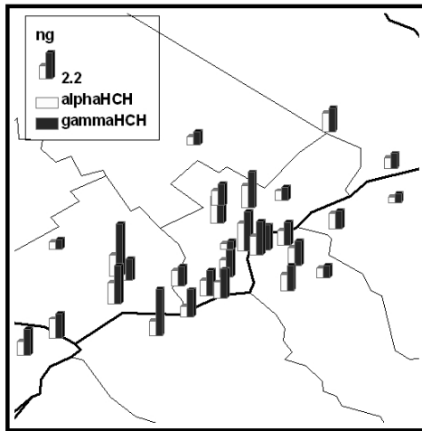
a) \alpha -HCH and \gamma -HCH
